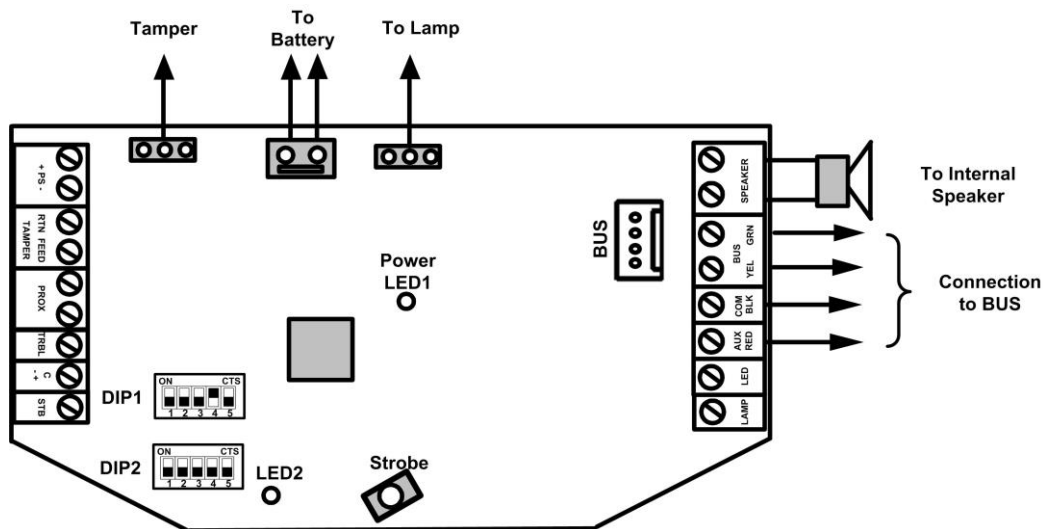
Figure 2: BUS Wiring
